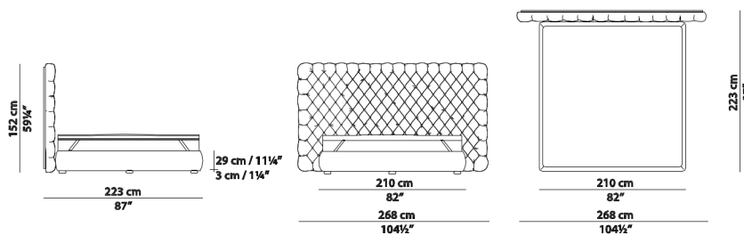
268 x 223 h 152 ( rete/spring 200 x 200 ) Letto / Bed
