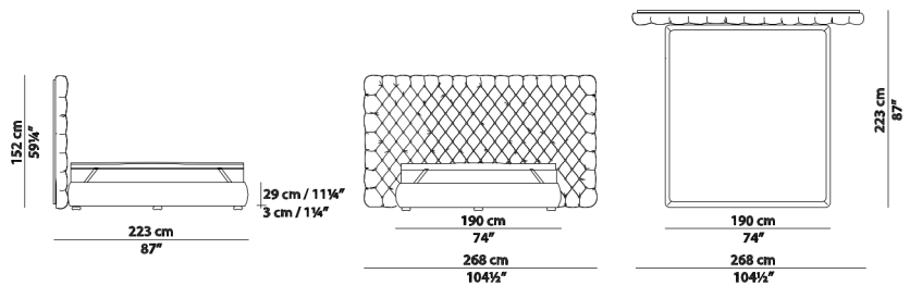
268 x 223 h 152 ( rete/spring 180 x 200 ) Letto / Bed
